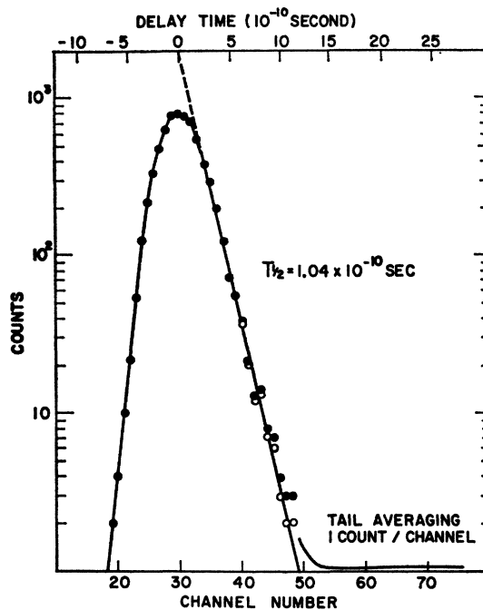
FIG. 26. Time spectrum of coincidences between conversion lines and \gamma rays above \sim 700 keV obtained in triple coincidence with a \beta ray in the decay \text{Tb}^{160} \rightarrow \text{Dy}^{160} .
