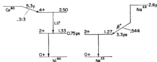
FIG. 27. Decay schemes of Na 22 and Co 60 . Half-lives of 2+ states taken from reference 11.
